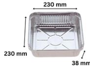
BK 7223 Aluminum Foil Square [360] 230mm x 230mm x 38mm Qty: 200 PCS/CTN
